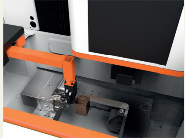
WorkPal 1 Application example: B-axis for Wire-cutting EDM (wire EDM).
