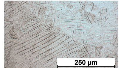
Microstructure as built
